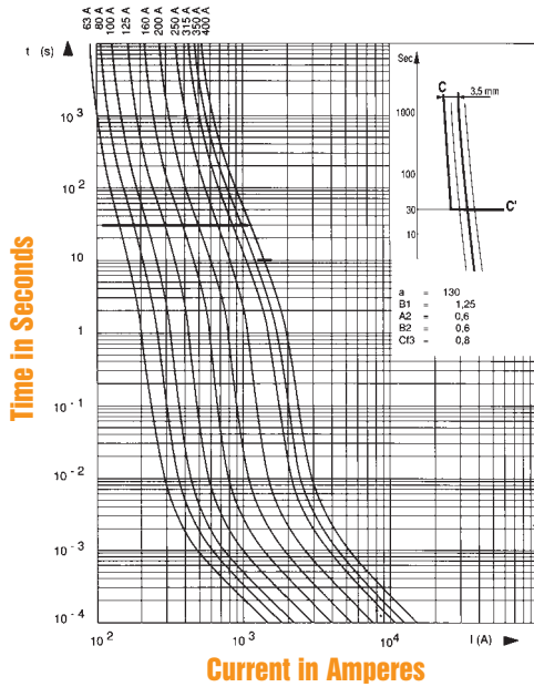
Melting Time – Current Data
