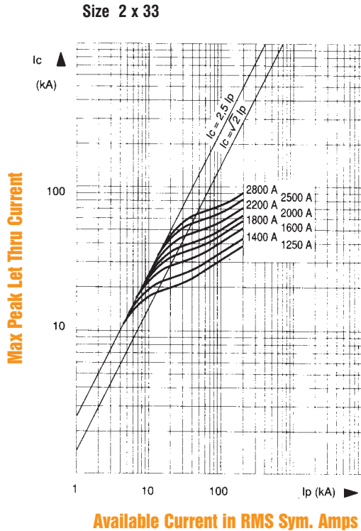
Peak let-thru Data 2X33
