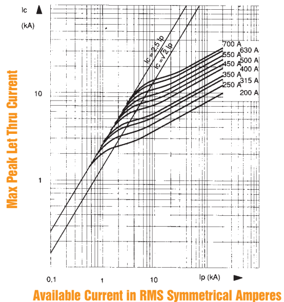
Peak Let-Thru Current Data
