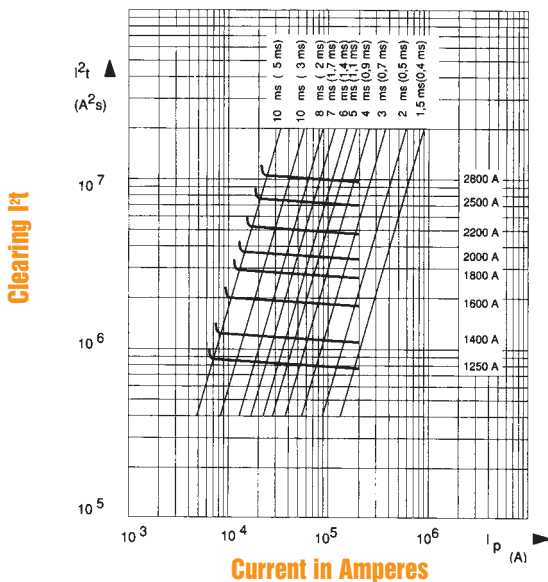
Clearing I 2 t Data 2X33
