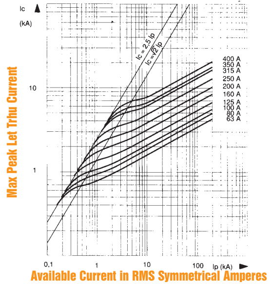
Peak Let-Thru Current Data
