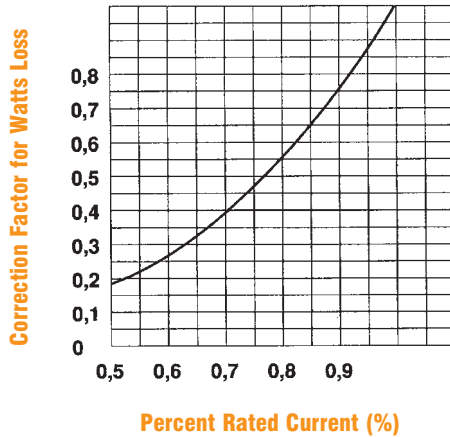
Watts Loss vs. % Rated Current
