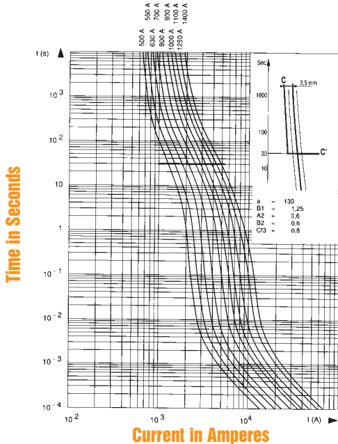
Melting Time – Current Data
