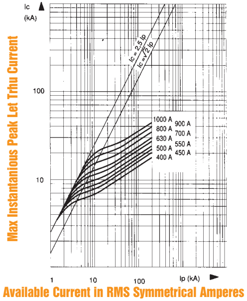
Peak Let-Thru Current Data
