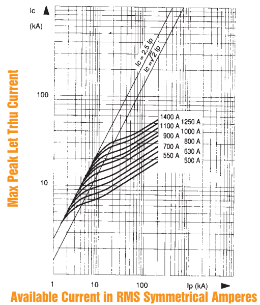
Peak Let-Thru Current Data
