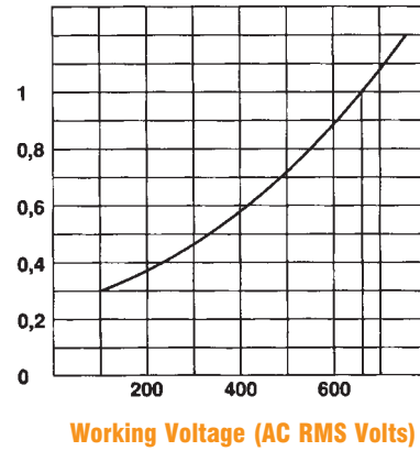
Clearing I 2 t vs. Operating Voltage
