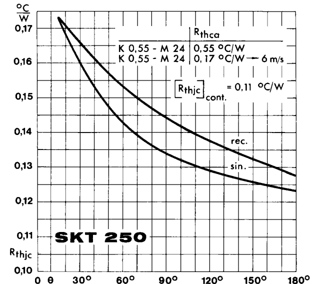
Fig. 5 a Thermal resistance vs. conduction angle
